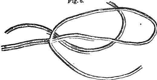
PALEOCHORDA MINOR. (One half nat. size.)
